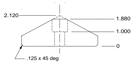
V-Block Profile
