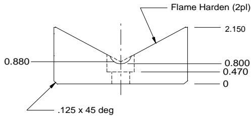
U-Block Profile
